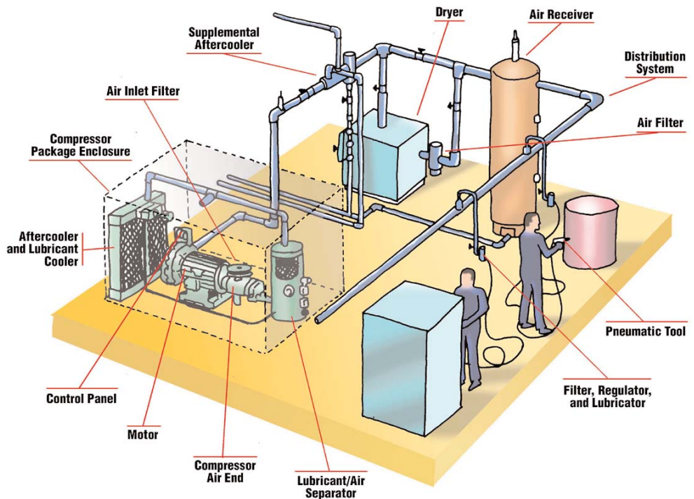
Figure 1 Basic compressed air system
