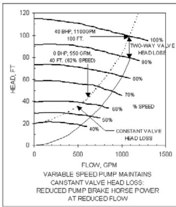
Figure 4. Typical Head / Capacity Curves For A Centrifugal Pump
