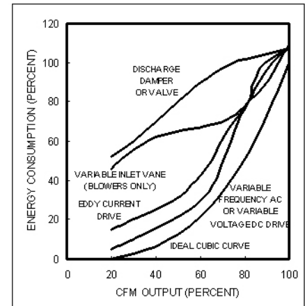
Figure 3. Typical Energy Requirements of A Centrifugal Fan Or Pump
